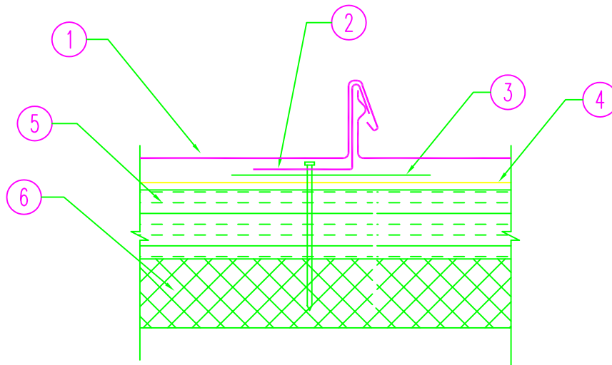
ALTERNATE DETAIL SECTION AT RIGID INSULATION OVER WOOD DECK
