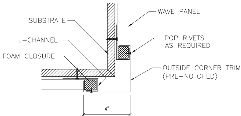
OUTSIDE CORNER DETAIL
