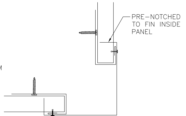
ENLARGED OUTSIDE CORNER DETAIL
