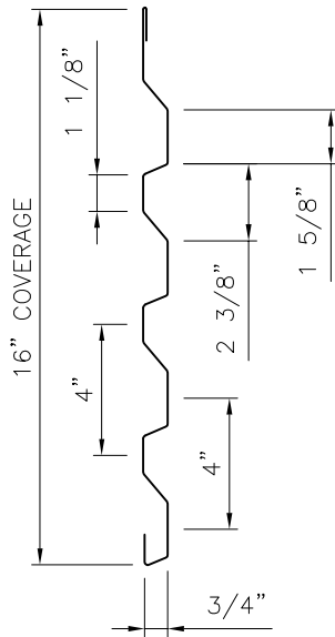
WAVE PANEL PROFILE Standard Width(s)- 16"
