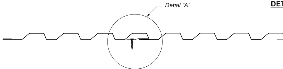
SEAM ENGAGEMENT
