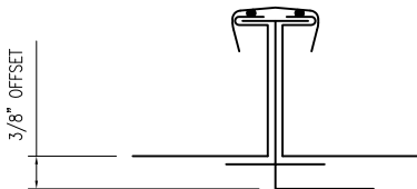
BEFORE SEAMING
