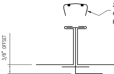
SEAM ENGAGEMENT
