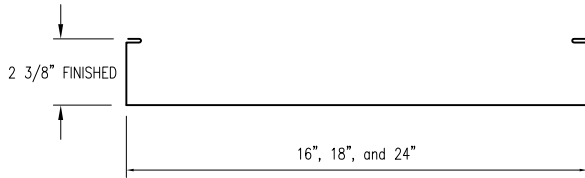
238T PANEL PROFILE Standard Width- 16"-18" and 24"
