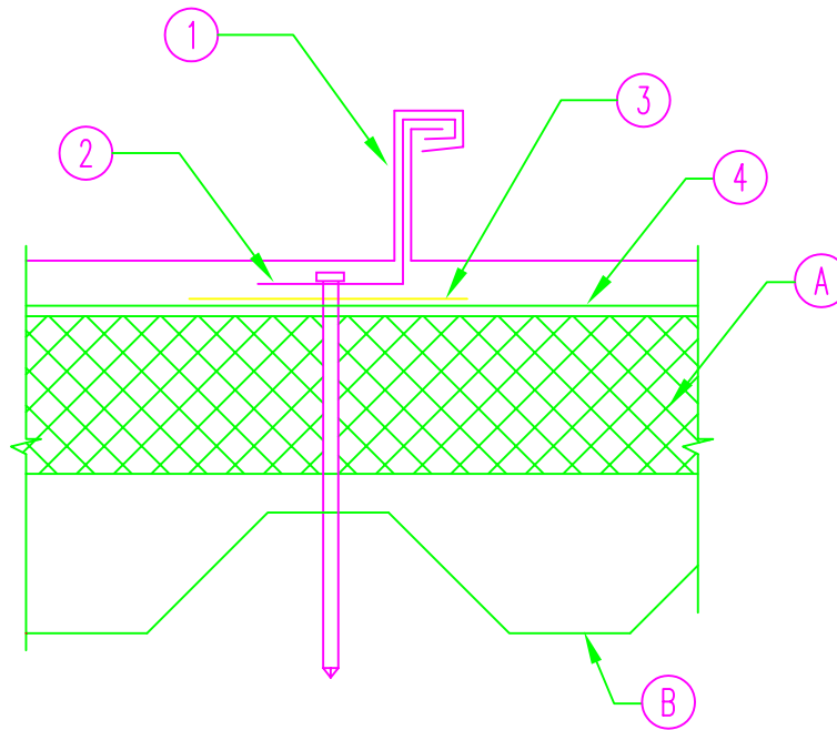
SECTION SHOWING INSTALLATION OVER INSULATION
