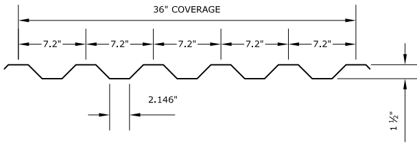
7.2" RIB PANEL PROFILE Standard Width(s)- 38 1/4" (36" Coverage)
