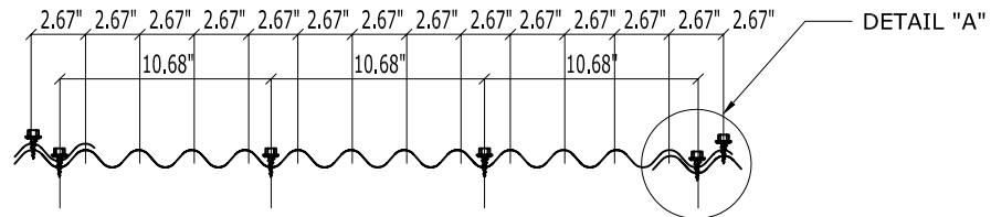
PANEL FASTENER LOCATIONS @ MIDDLE OF PANEL
