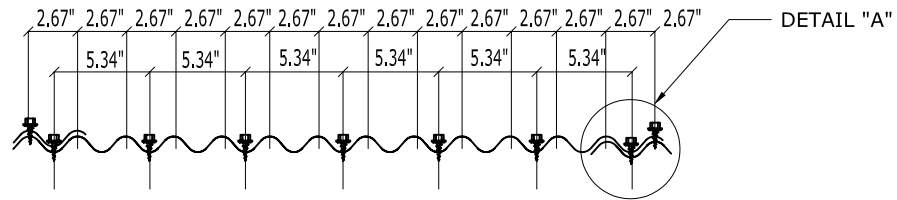
PANEL FASTENER LOCATIONS @ PANEL ENDS
