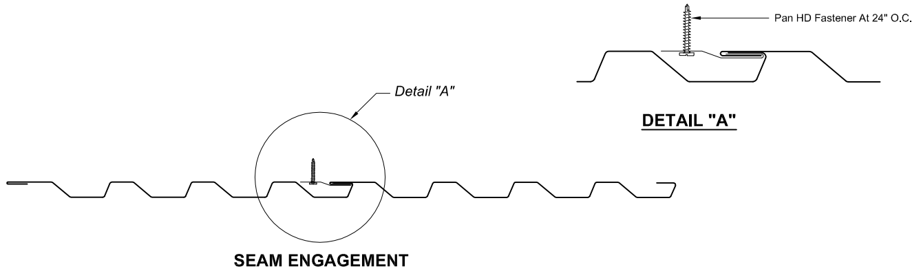
SEAM ENGAGEMENT
