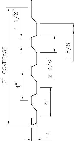
WAVE PROFILE Width- 16"
