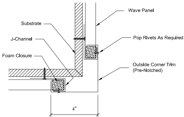
OUTSIDE CORNER DETAIL
