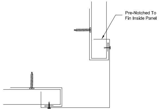
ENLARGED OUTSIDE CORNER DETAIL
