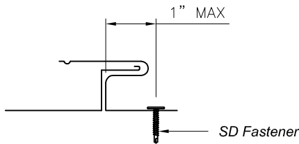
UD LINER PANEL PROFILE (SMOOTH) ~VEE GROOVES @ 6" O.C.~ Standard Width(s)- 18"
