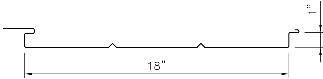
UD LINER PANEL PROFILE (SMOOTH) ~VEE GROOVES @ 6" O.C.~ Standard Width(s)- 18"
