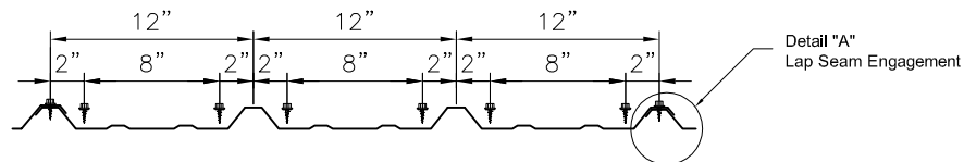
PANEL FASTENER LOCATIONS AT PANEL ENDS
