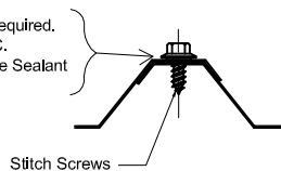
DETAIL "A" LAP SEAM ENGAGEMENT
