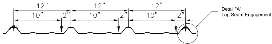
PANEL FASTENER LOCATIONS AT MIDDLE OF PANEL
