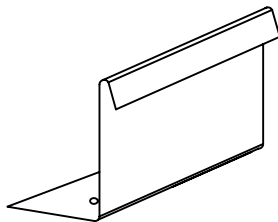
24 GAUGE INSTALOC CLIP (2 FASTENERS)
