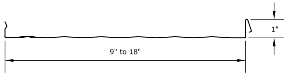
INSTALOC PROFILE W/ STRIATIONS
