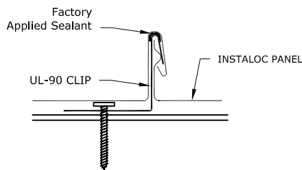
INSTALOC PANEL SEAM
