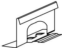
STANDARD CLIP (ONE FASTENER) 16 GAUGE
