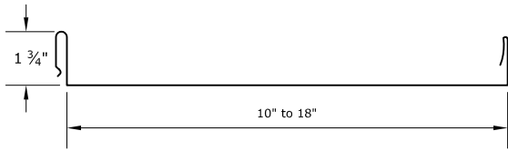
PERMASEAM PANEL PROFILE (SMOOTH) Standard Width(s)- 10", 12", 16", and 18"
