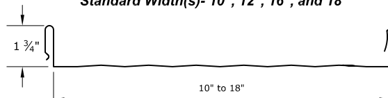
PERMASEAM PANEL PROFILE (STRIATED) Standard Width(s)- 10", 12", 16", and 18"
