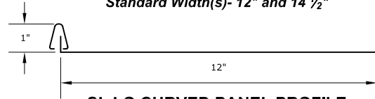
SL LO CURVED PANEL PROFILE 12" ONLY (Minimum Radius= 2'-6")
