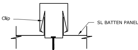
SL BATTEN PANEL SEAM
