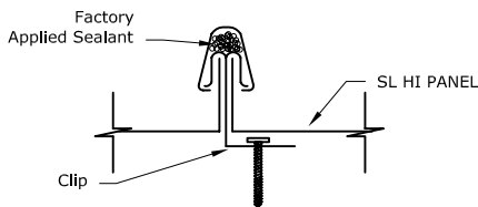
SL HI PANEL CLIP
