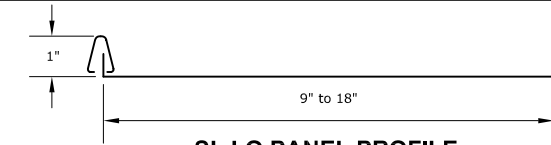
SL LO PANEL PROFILE Standard Width(s)- 12" and 14 1/2"
