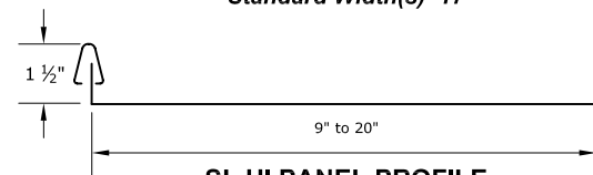
SL HI PANEL PROFILE Standard Width(s)- 13 1/2" and 18"
