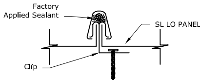
SL LO & SL LO CURVED PANEL SEAM
