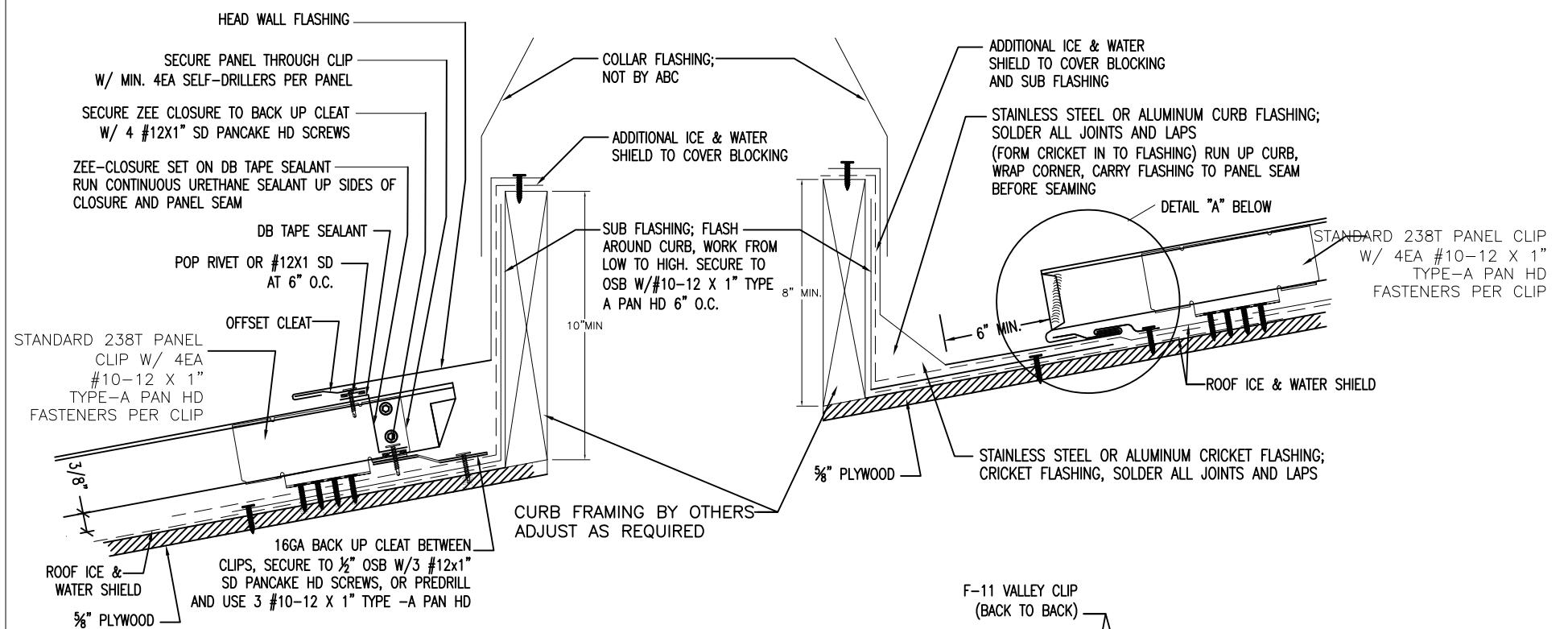
TYP CURB DETAIL SECTION B-B
