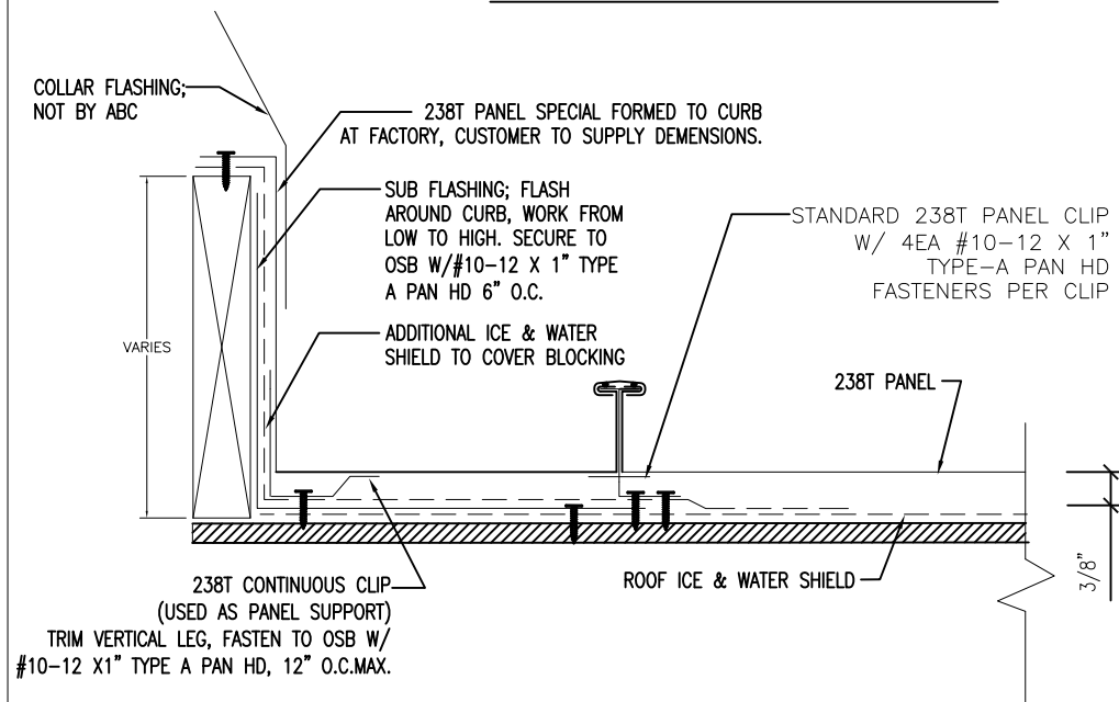
TYP CURB DETAIL SECTION B-B
