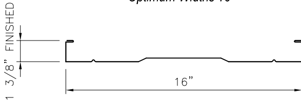
PLANK & PENCIL PROFILE Optimum Widths 16"
