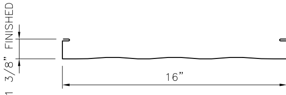
STRIATED PROFILE Optimum Widths 16"
