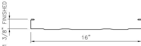
STIFFENER RIB PROFILE WITH OPTIONAL CLIP OFFSET Optimum Widths 16"
