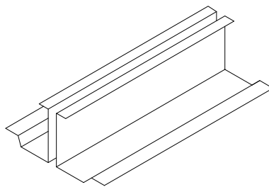
MULTISPAN CLIP 2-Piece 24 GA (Standard) 22 GA (Available) (Continuous or 8" long clips)
