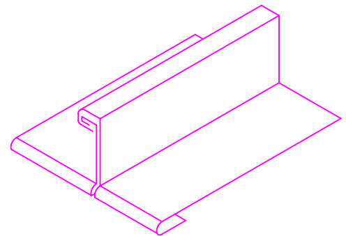
PANEL END AFTER FOLDING HEM
