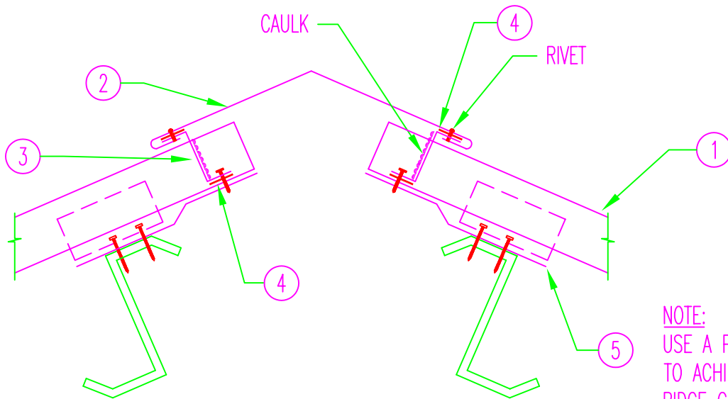
SECTION HIP/RIDGE
