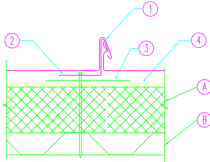
SECTION AT RIGID INSULATION
