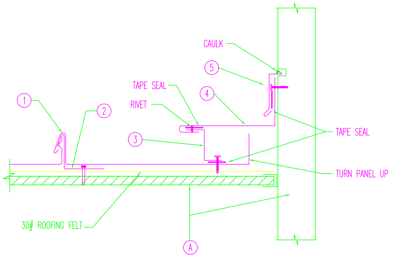
SECTION AT SIDEWALL
