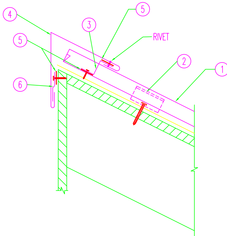
SECTION AT HIGH EAVE
