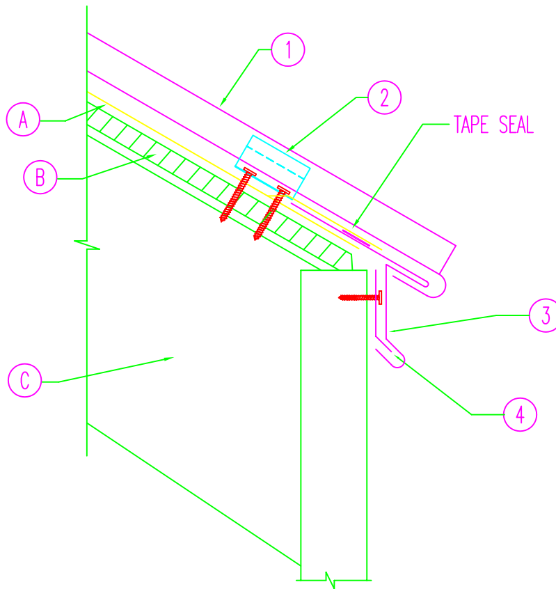
EAVE DETAIL
