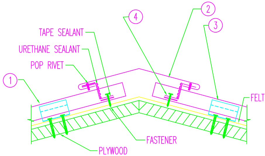
TYPICAL SECTION AT RIDGE/HIP
