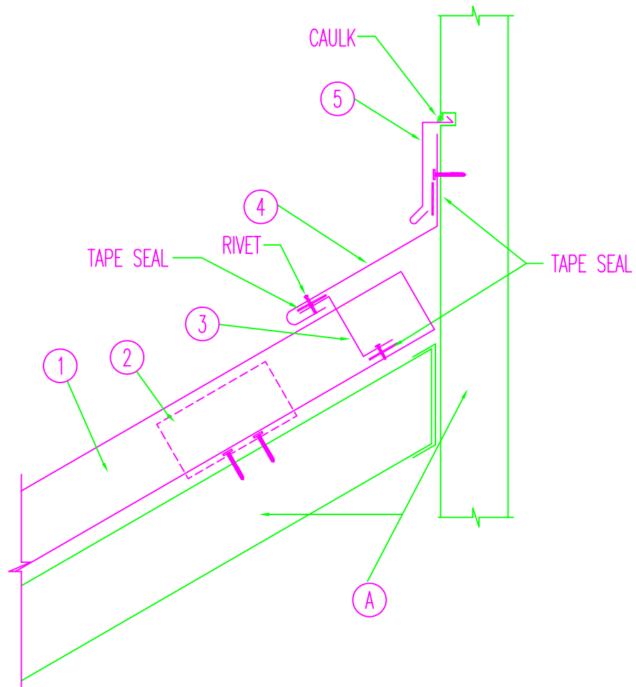
SECTION AT HEADWALL
