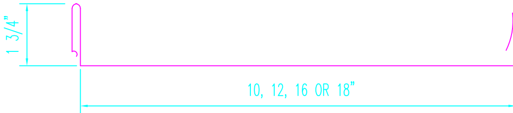
PERMASEAM PANEL PROFILE
