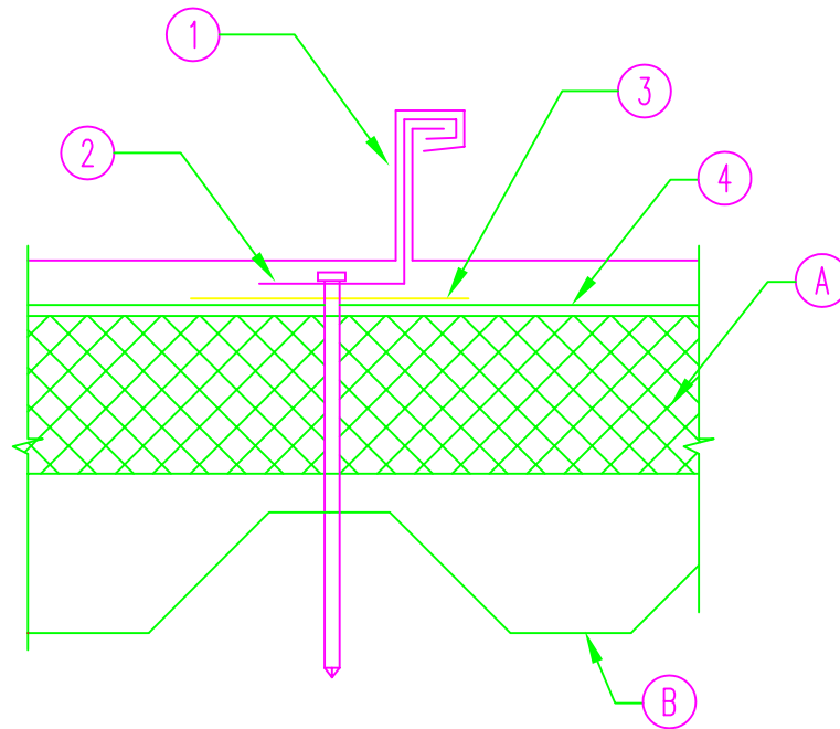
SECTION SHOWING INSTALLATION OVER INSULATION
