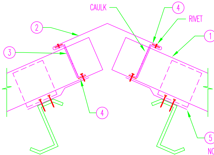
SECTION HIP/RIDGE
